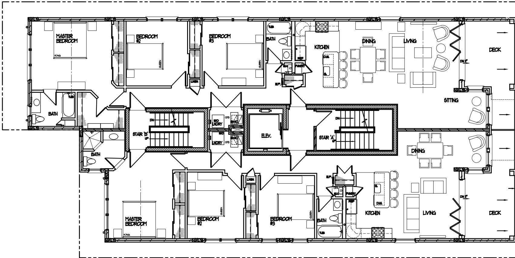
FIRST FLOOR PLAN SCALE: 3/16" = 1'-0"
