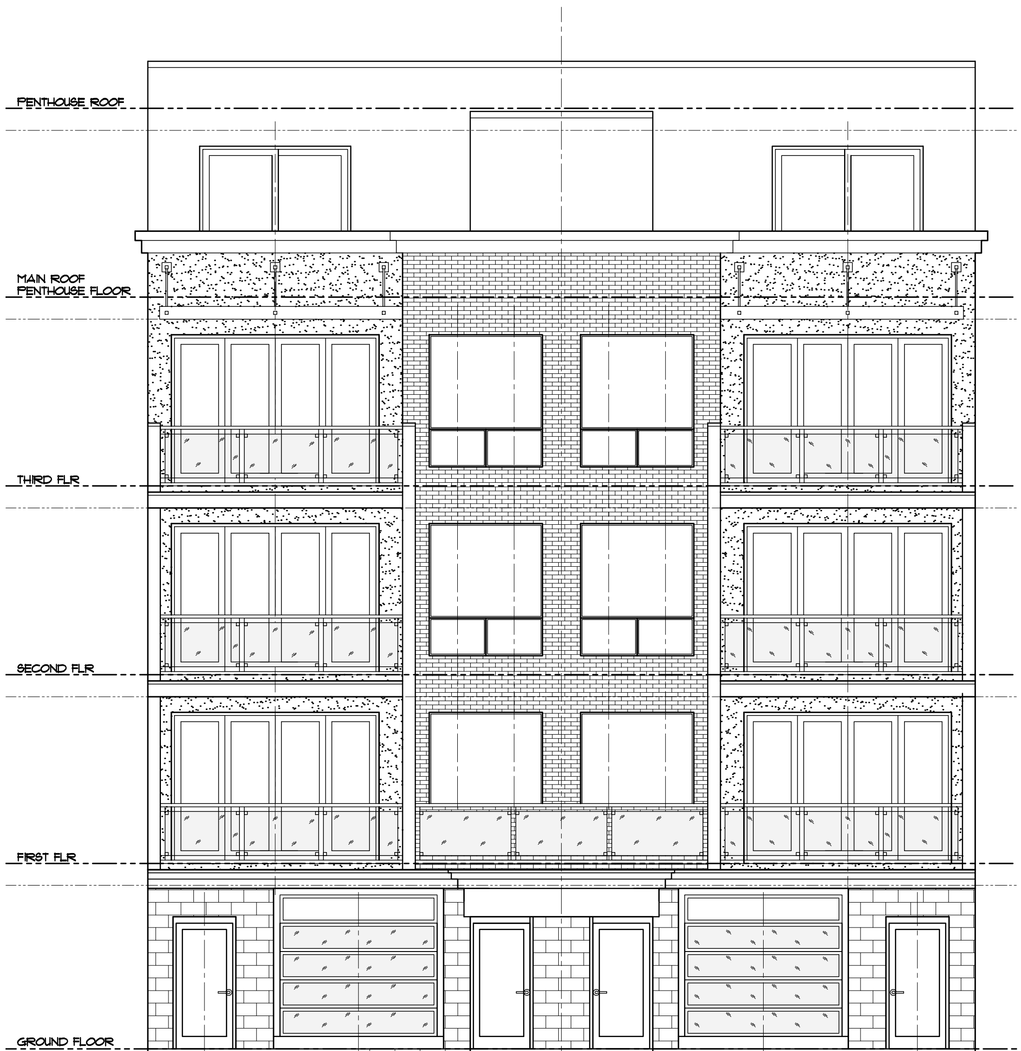
FRONT ELEVATION - EAST
