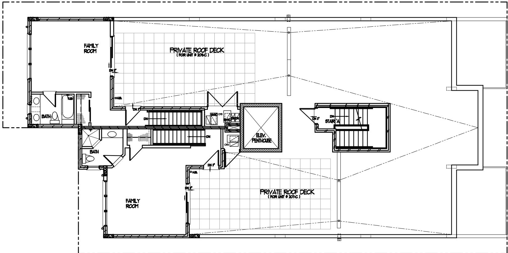
PENTHOUSE PLAN SCALE 3/8" = 1'-0"
