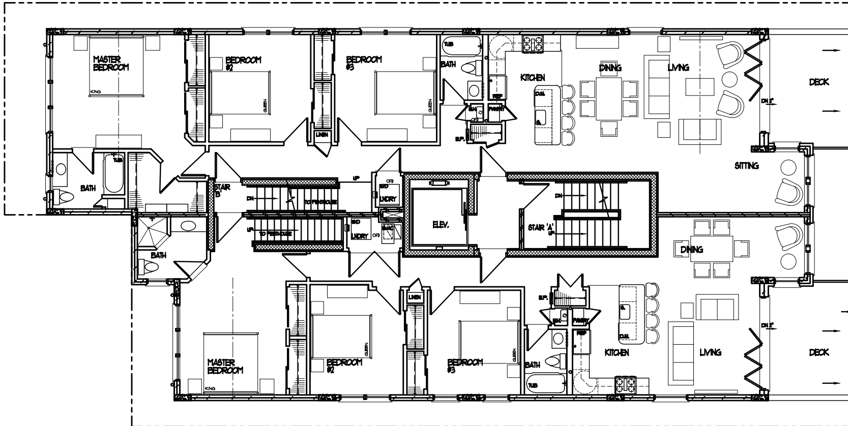
THIRD FLOOR PLAN - DUPLEX APTMENTS W/ PENTHOUSE ABOVE SCALE: 3/16" = 1'-0"
